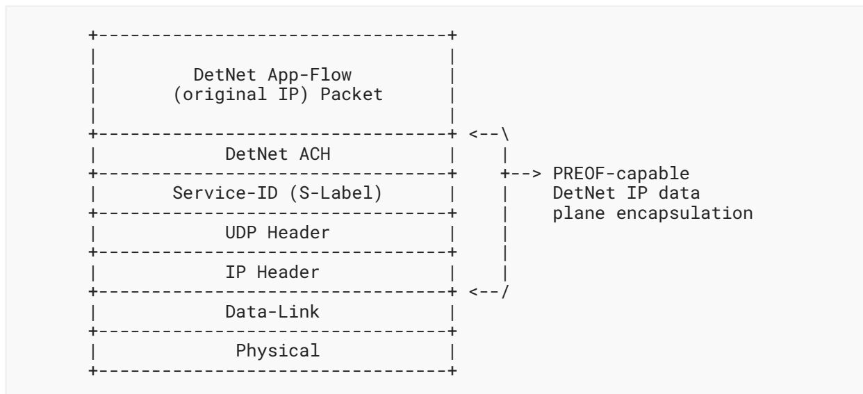
Figure 1: DetNet Associated Channel Header Format
