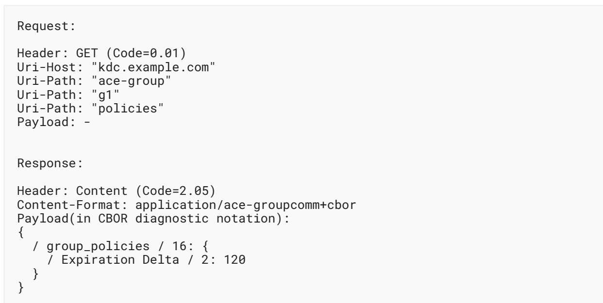
Figure 24: Example of Policies Request-Response
