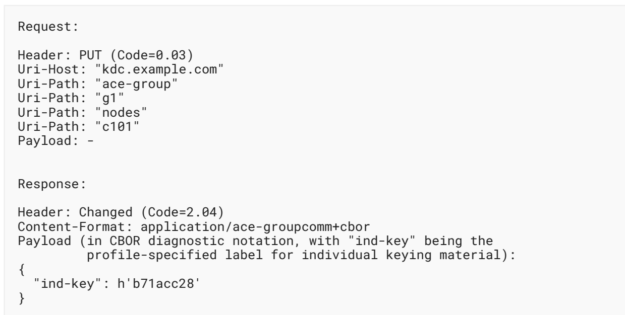
Figure 30: Example of Key Renewal Request-Response
